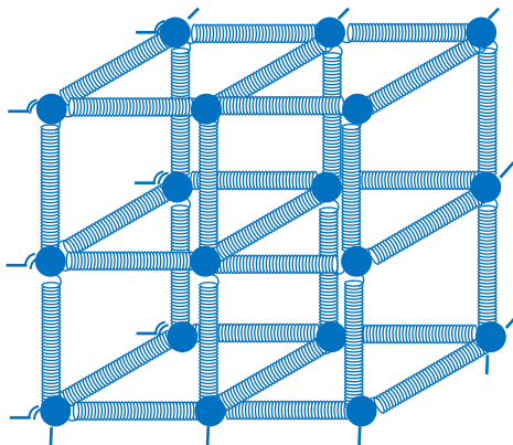
Figure : Spring-ball model for the illustration of elastic behaviour of solids
