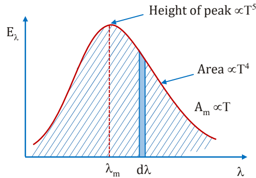
Spectral energy distribution curve ( E_\lambda - \lambda )
