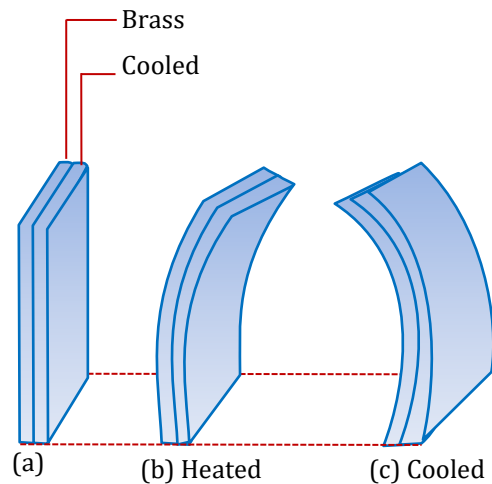
(a) A bimetallic strip and how it behaves when (b) heated and (c) cooled
